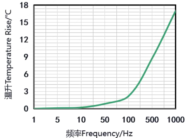
Temperature Rise vs. Drive Frequency
